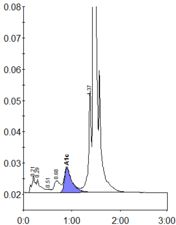
Peak table - ID: 11086995
