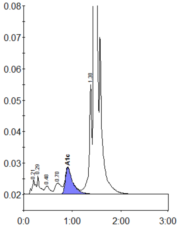
Peak table - ID: 11071915
