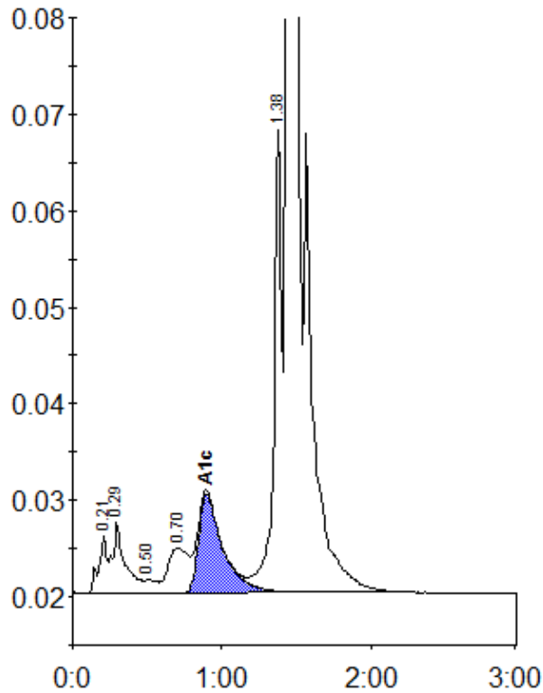
Peak table - ID: 11099366
