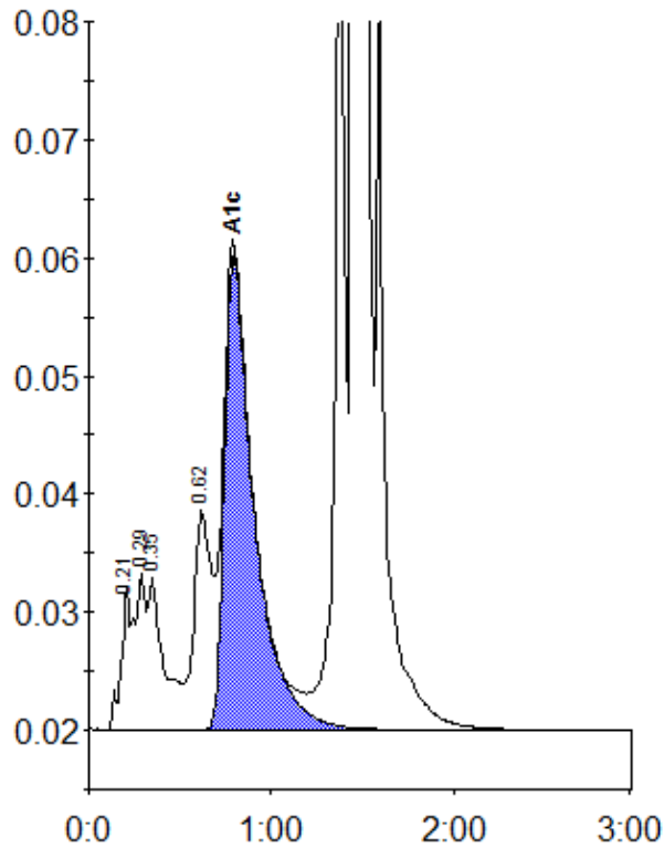
Peak table - ID: 11122464
