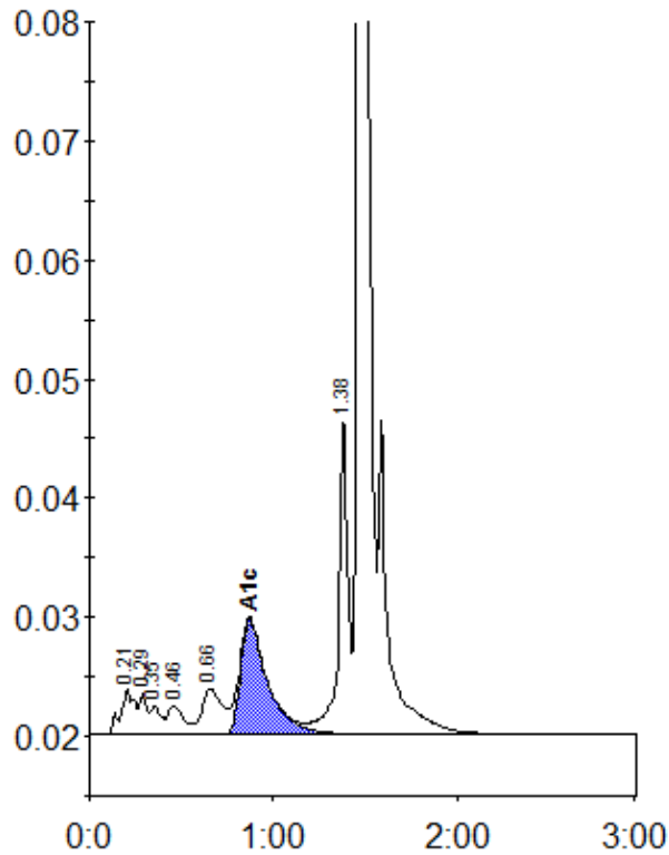
Peak table - ID: 11128351
