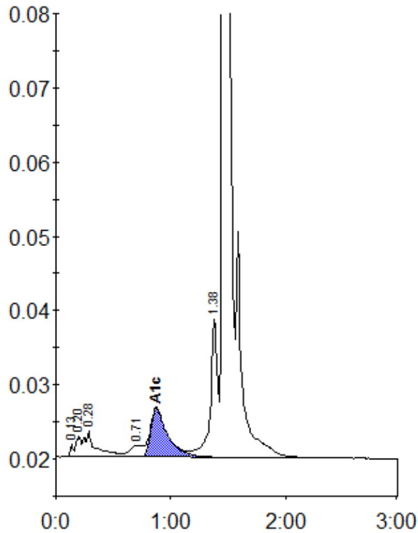
Peak table - ID: 10960419
