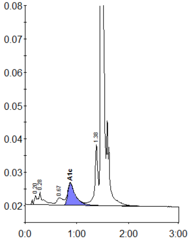
Peak table - ID: 10863732
