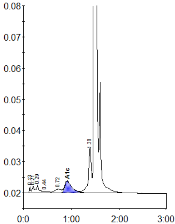
Peak table - ID: 726880
