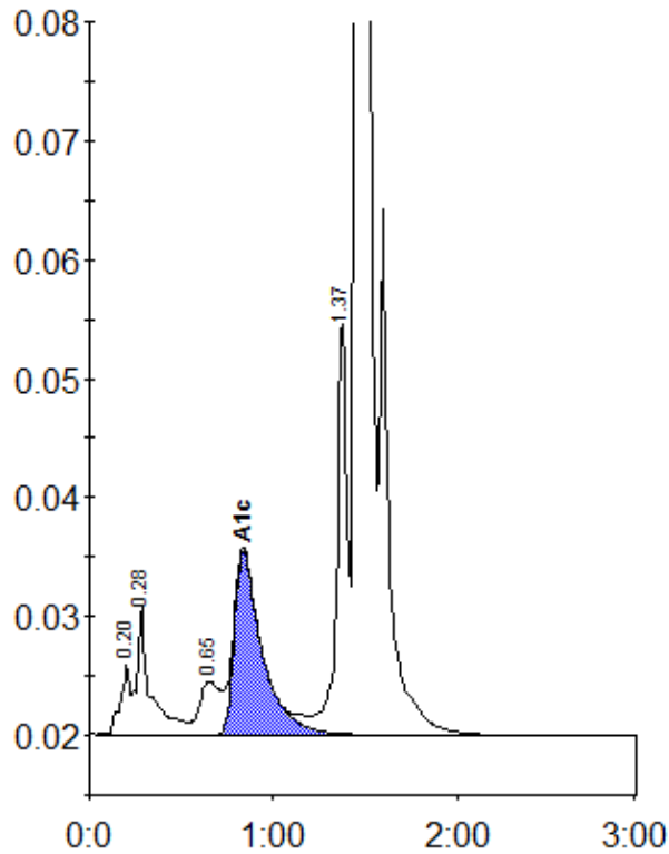
Peak table - ID: 10981967
