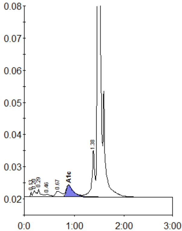
Peak table - ID: 11009903
