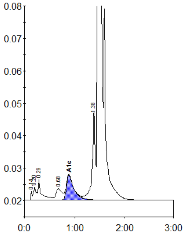
Peak table - ID: 11009963
