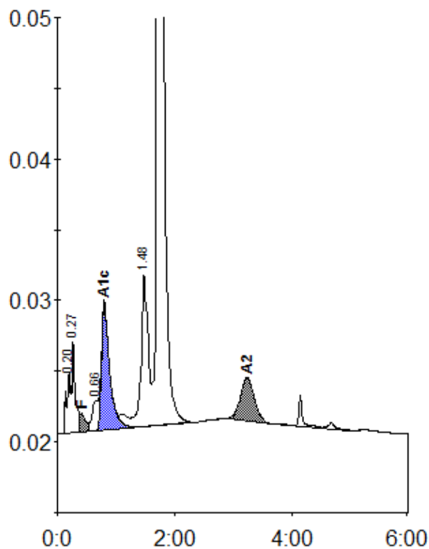
Peak table - ID: 11011271
