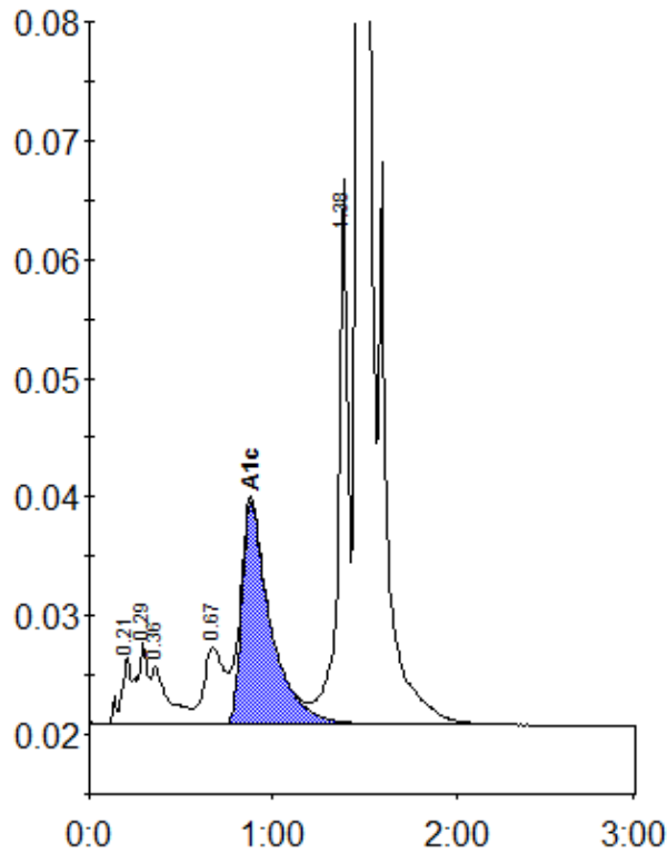
Peak table - ID: 10972973
