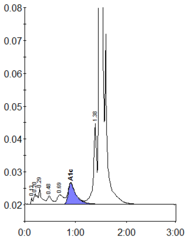
Peak table - ID: 10888323
