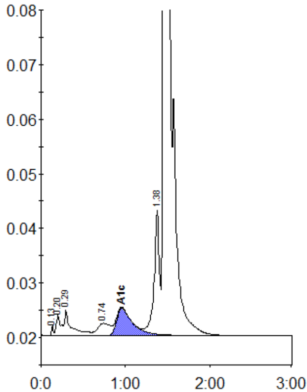
Peak table - ID: 10954175
