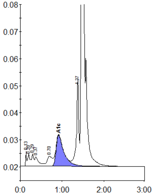
Peak table - ID: 10941657
