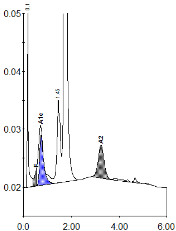
Peak table - ID: 100010285
