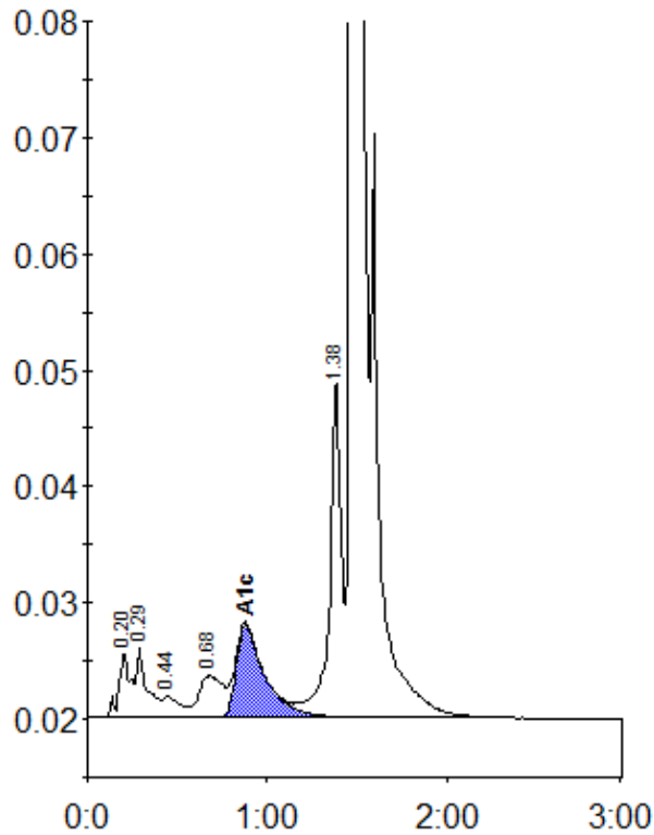
Peak table - ID: 10906500
