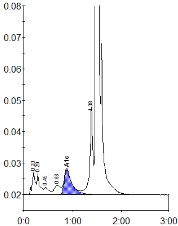
Peak table - ID: 10975824
