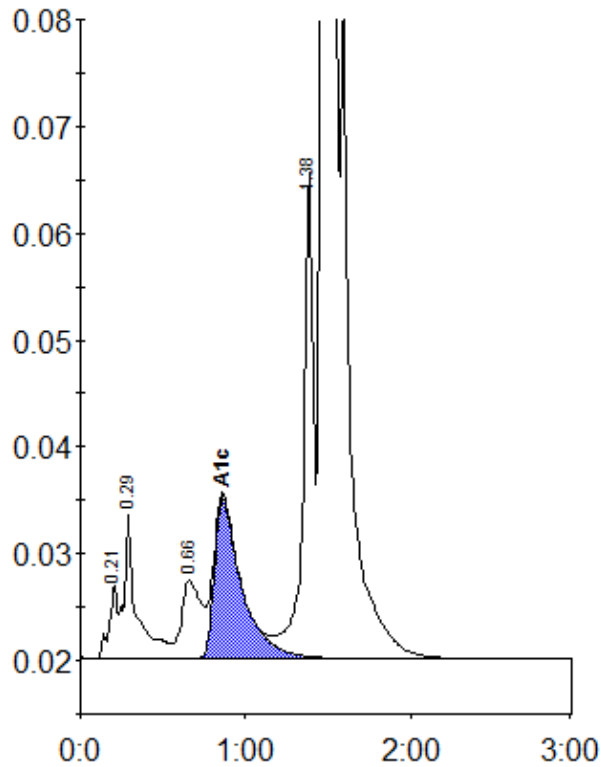
Peak table - ID: 10991342
