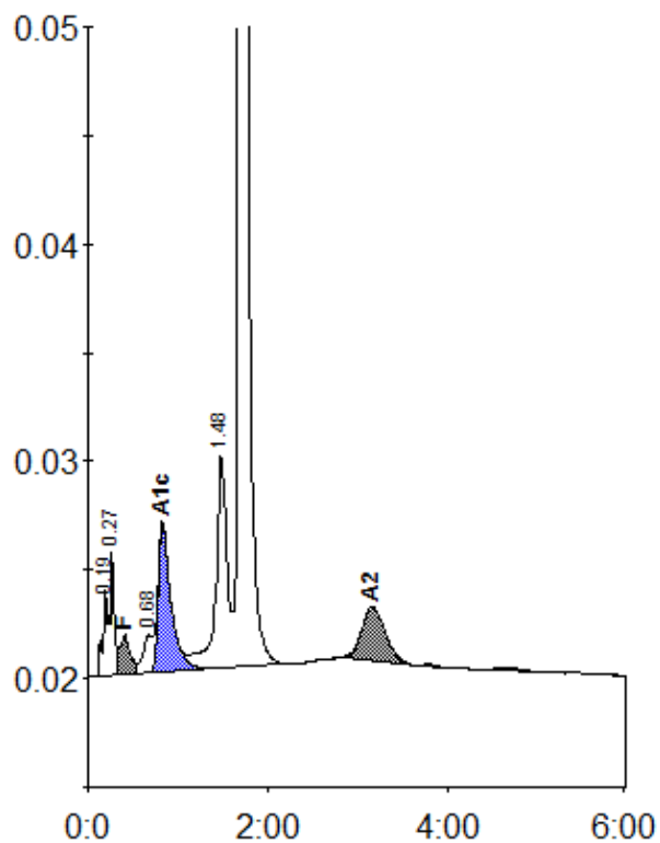
Peak table - ID: 10034538
