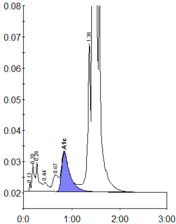
Peak table - ID: 10948218
