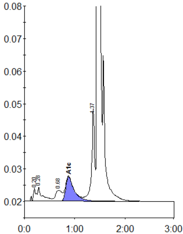
Peak table - ID: 10905052
