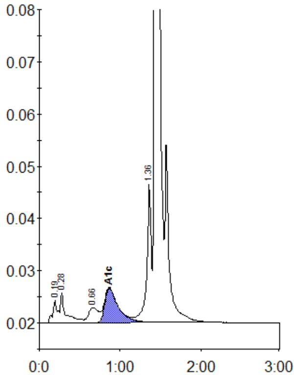
Peak table - ID: 10922439
