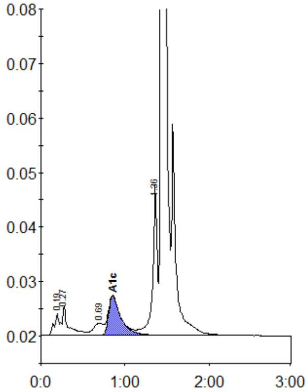
Peak table - ID: 10503616
