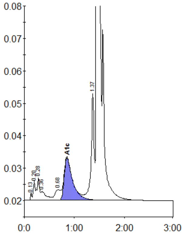
Peak table - ID: 10966644
