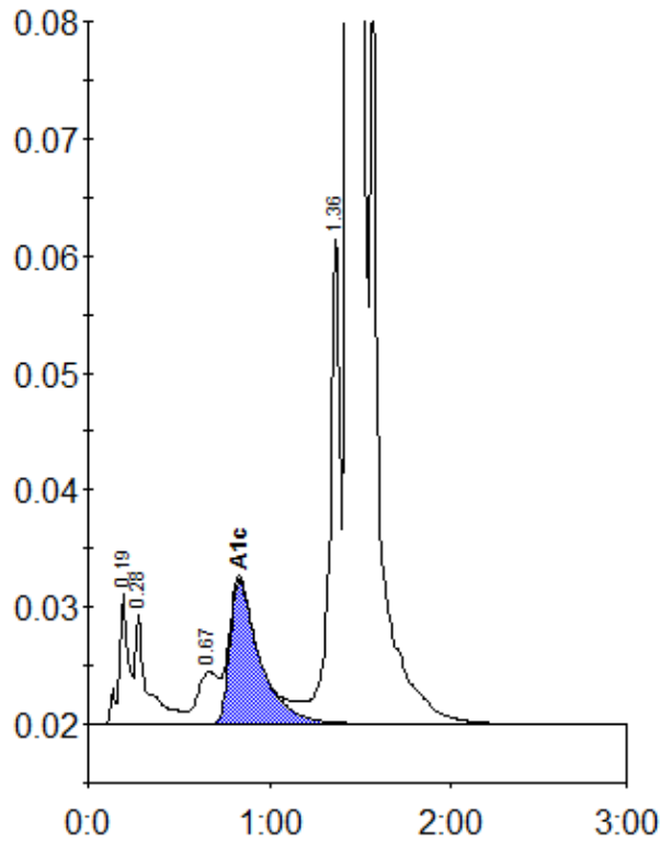
Peak table - ID: 10948332
