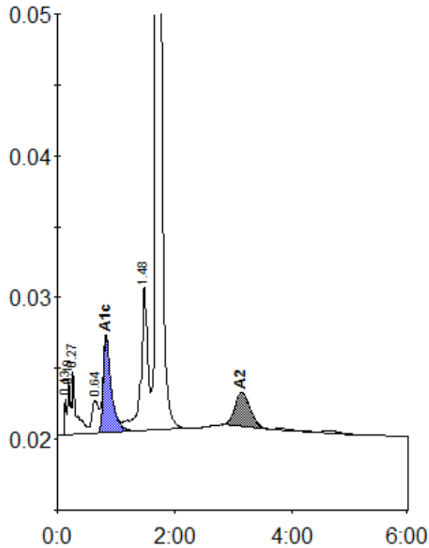
Peak table - ID: 10940485
