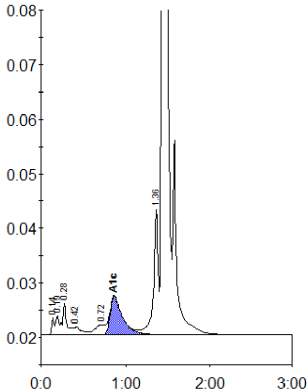
Peak table - ID: 10298133
