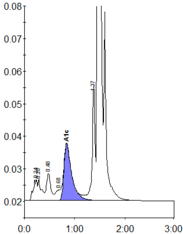
Peak table - ID: 10948998
