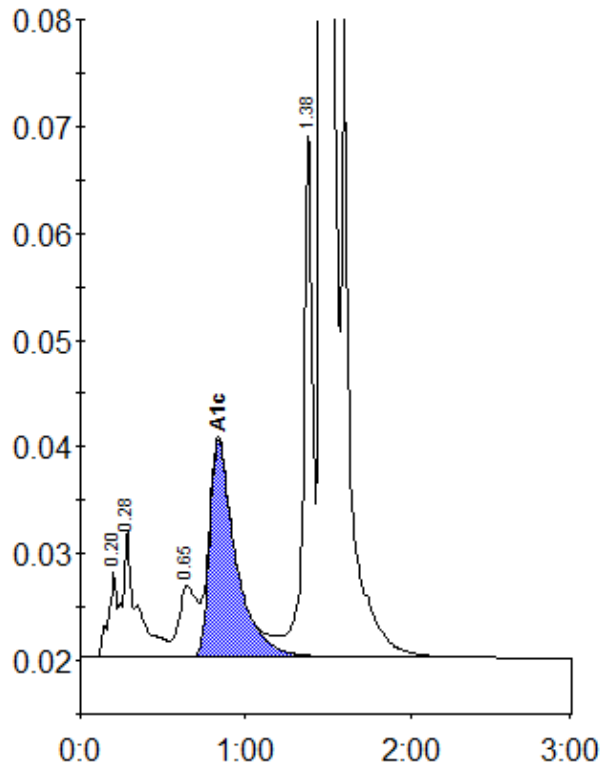
Peak table - ID: 10545201
