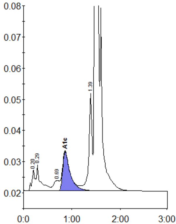
Peak table - ID: 10925834
