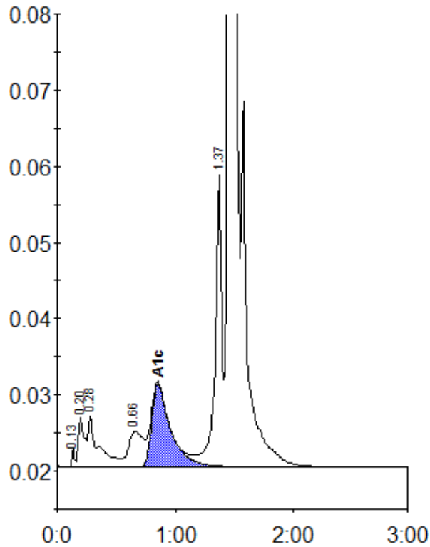
Peak table - ID: 10856290
