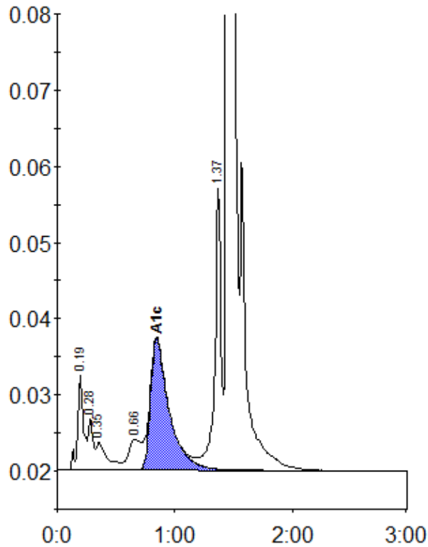
Peak table - ID: 10835937
