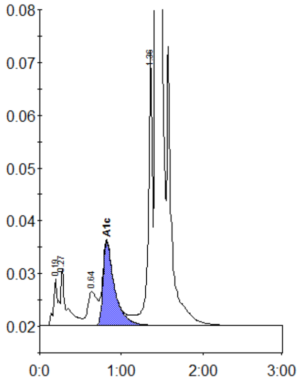
Peak table - ID: 10901629
