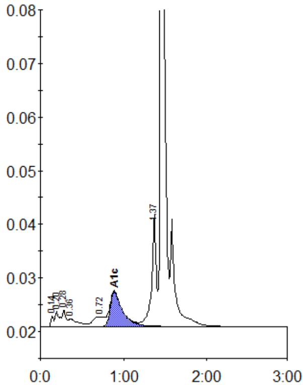
Peak table - ID: 10905347
