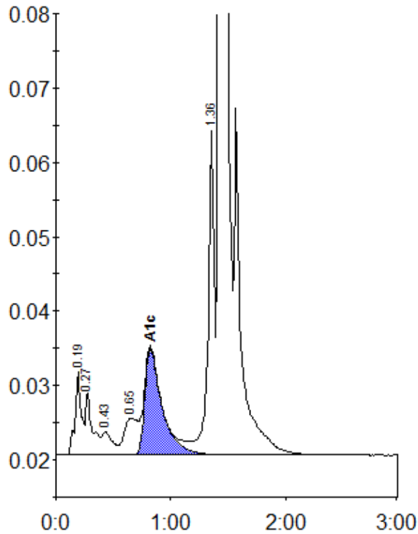
Peak table - ID: 10836900
