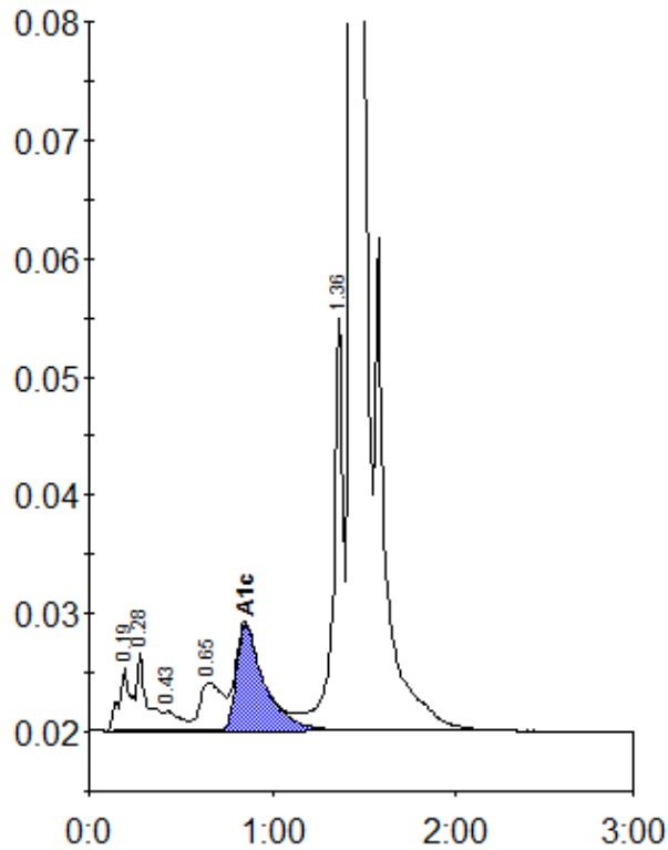
Peak table - ID: 10859223
