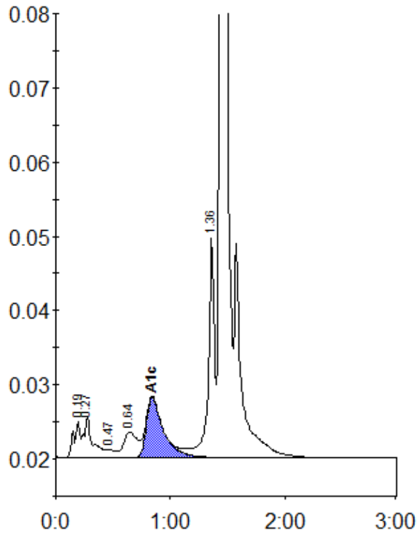
Peak table - ID: 10905599
