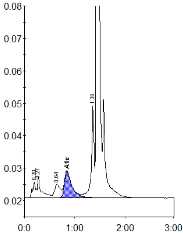
Peak table - ID: 10862640
