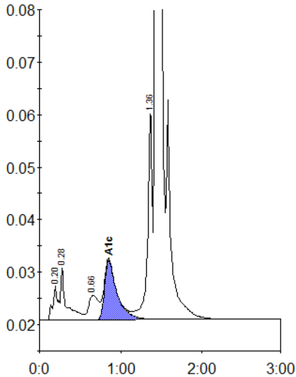
Peak table - ID: 10877990
