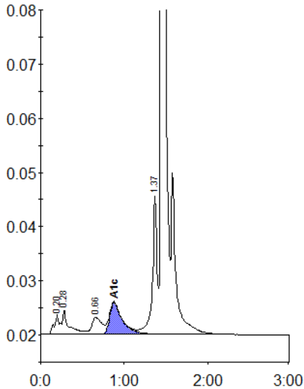
Peak table - ID: 10848982
