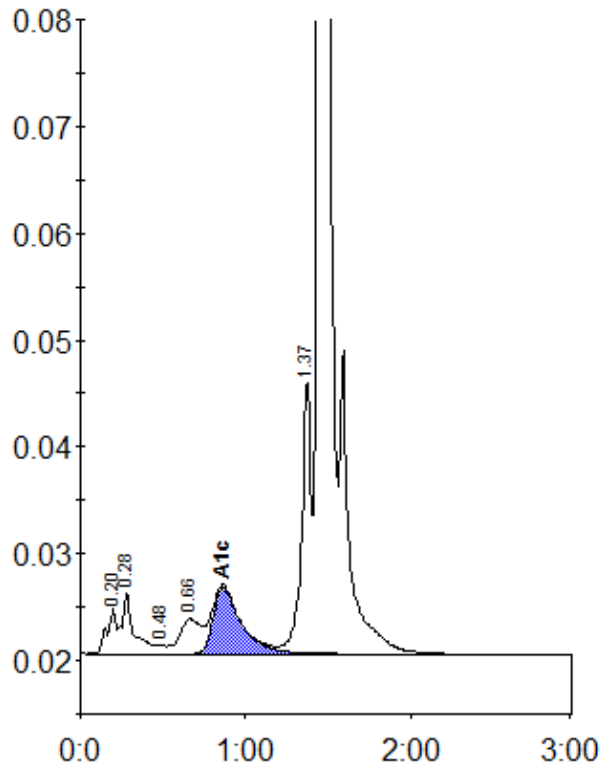
Peak table - ID: 10863087
