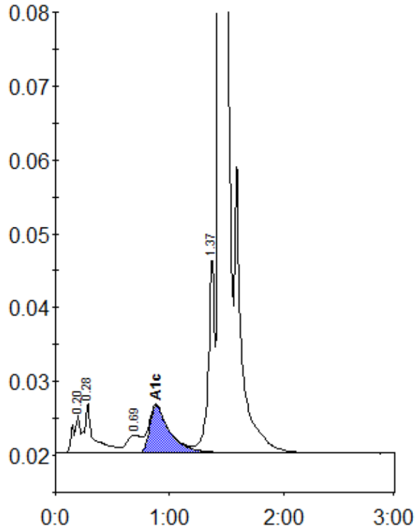
Peak table - ID: 10817907
