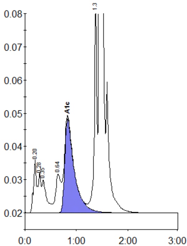
Peak table - ID: 10817853
