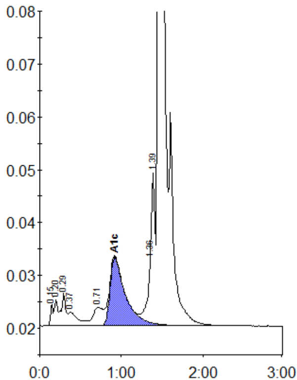
Peak table - ID: 10848932
