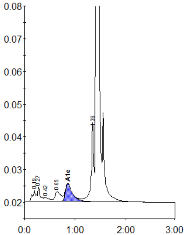
Peak table - ID: 10845599
