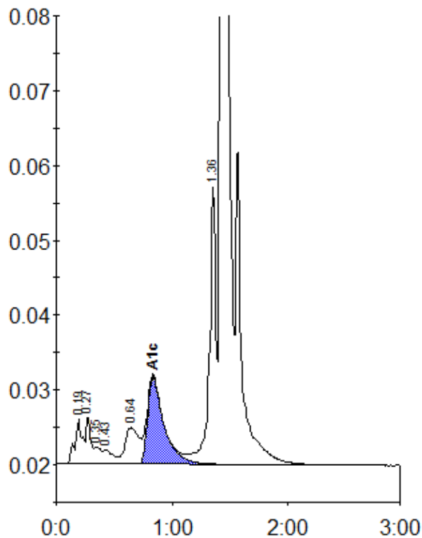
Peak table - ID: 10840179
