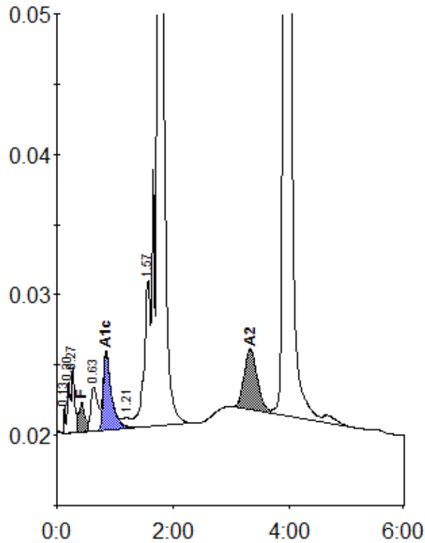
Peak table - ID: 10806864
