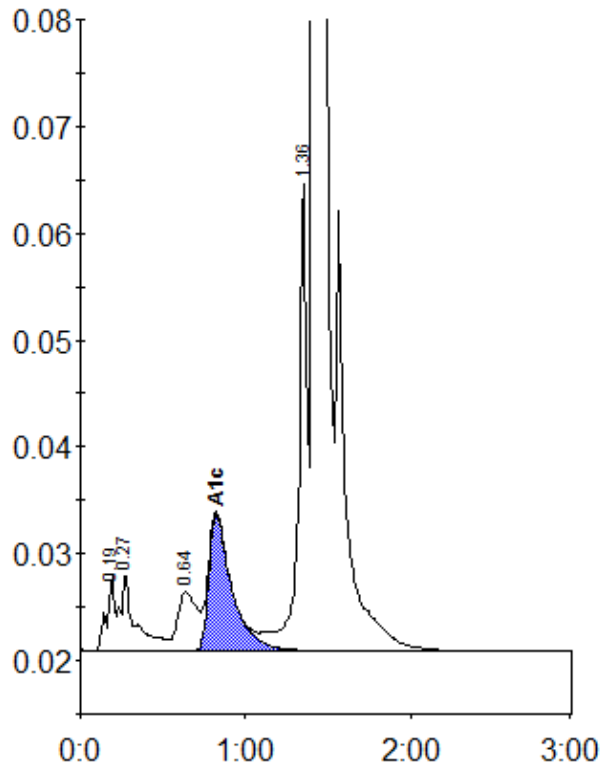
Peak table - ID: 10855178
